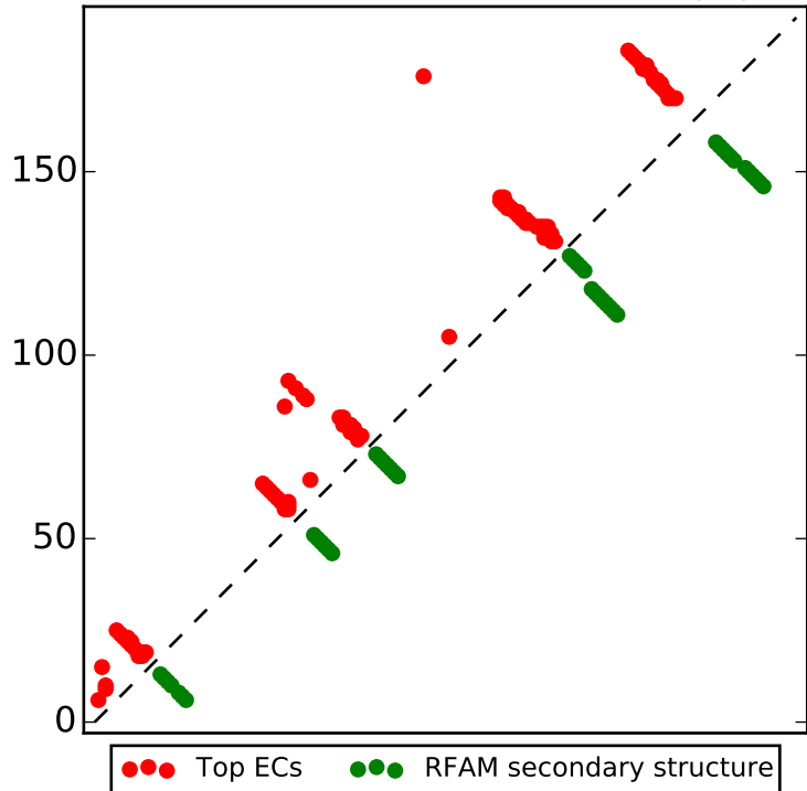
Top L/2 contacts for RF00004 with |i-j| > 4
