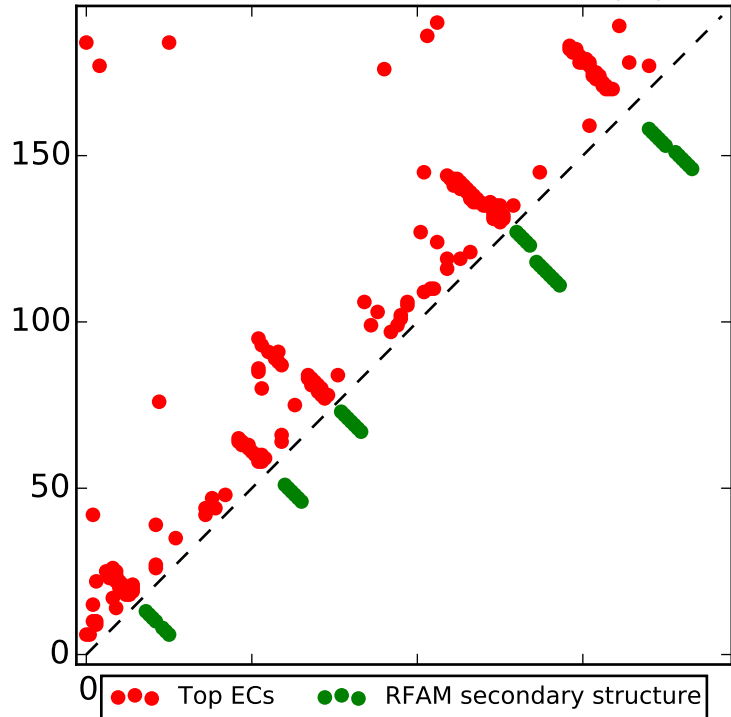
Top L contacts for RF00004 with |i-j| > 4
