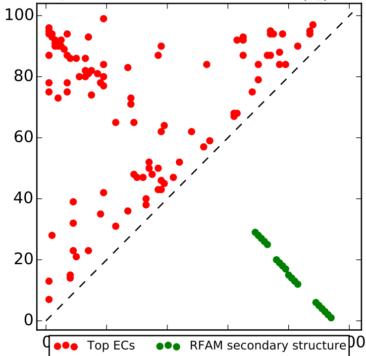
Top L contacts for RF00006 with |i-j| > 4
