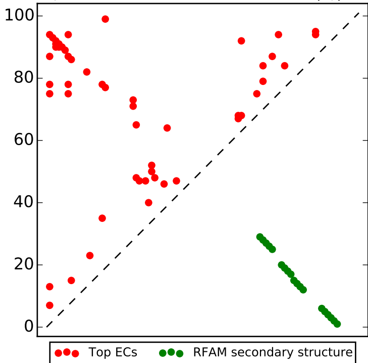
Top L/2 contacts for RF00006 with |i-j| > 4
