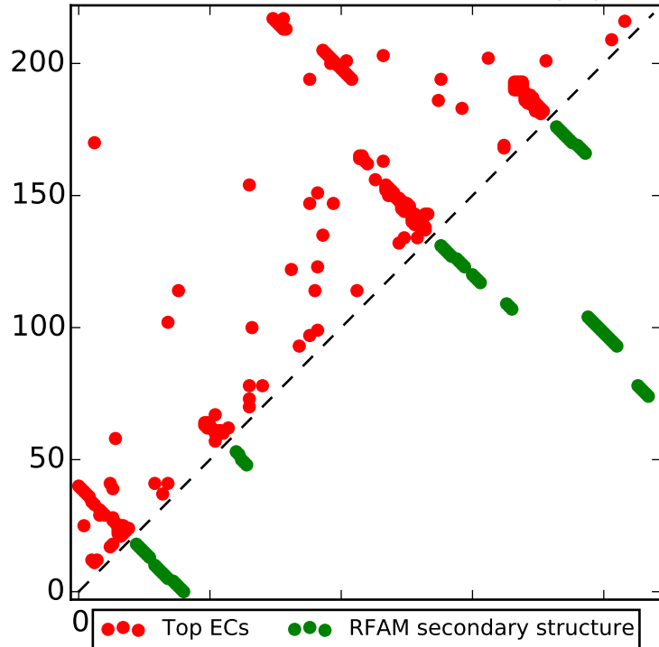
Top L contacts for RF00012 with |i-j| > 4
