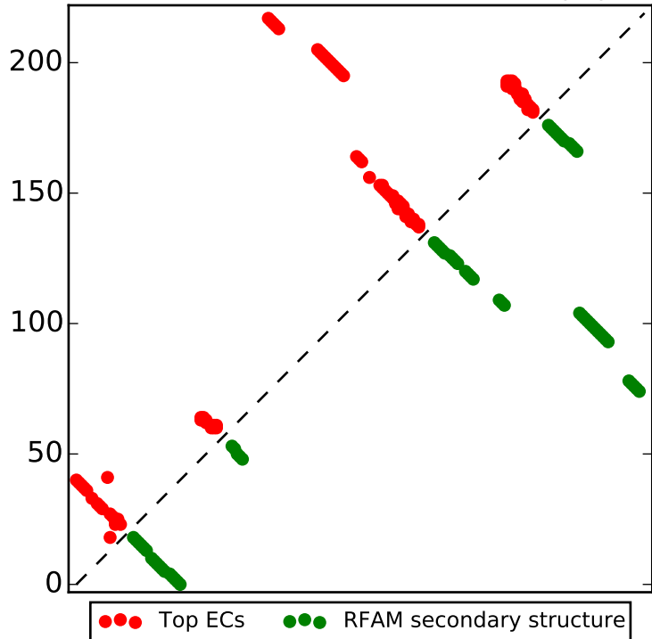
Top L/2 contacts for RF00012 with |i-j| > 4
