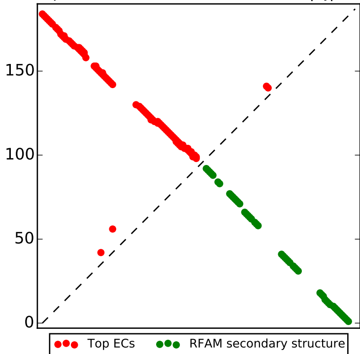
Top L/2 contacts for RF00013 with |i-j| > 4
