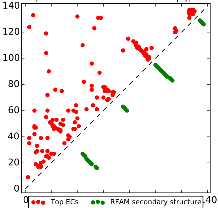
Top L contacts for RF00015 with |i-j| > 4
