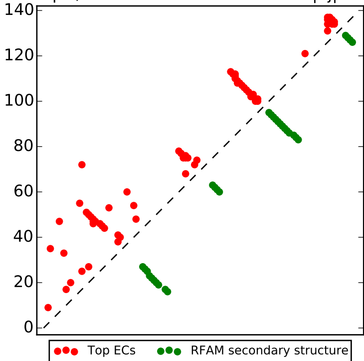
Top L/2 contacts for RF00015 with |i-j| > 4
