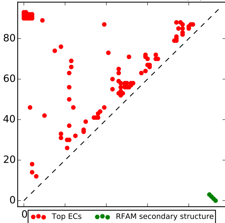
Top L contacts for RF00016 with |i-j| > 4
