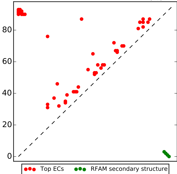
Top L/2 contacts for RF00016 with |i-j| > 4
