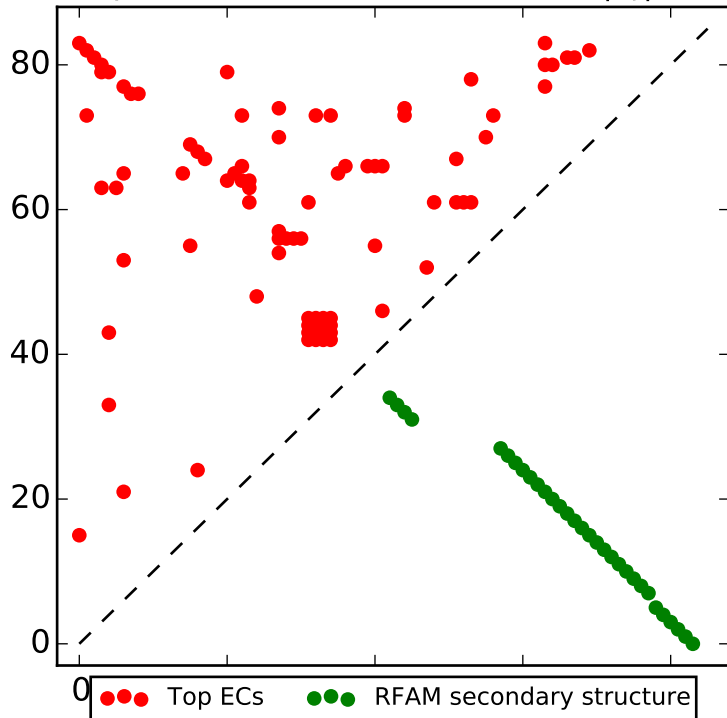
Top L contacts for RF00027 with |i-j| > 4
