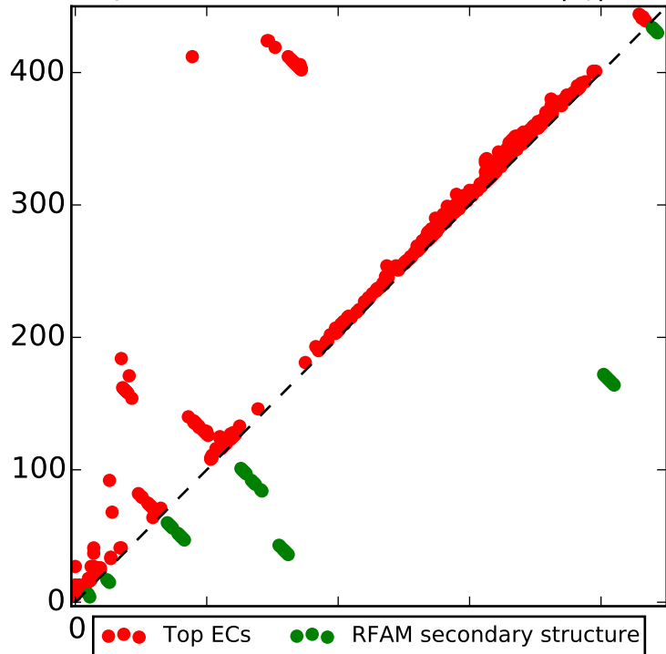
Top L contacts for RF00028 with |i-j| > 4
