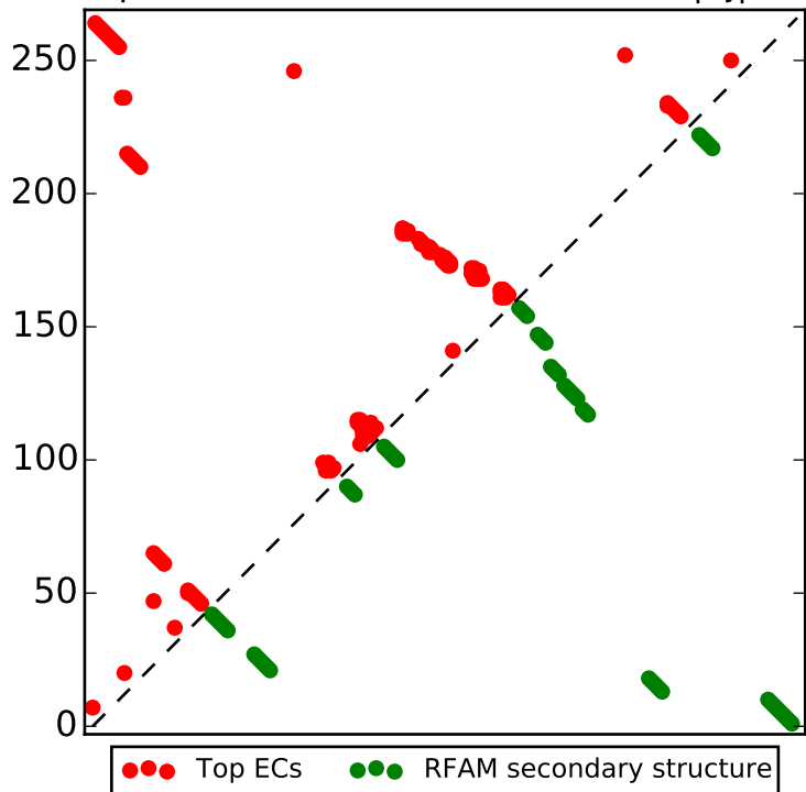
Top L/2 contacts for RF00030 with |i-j| > 4
