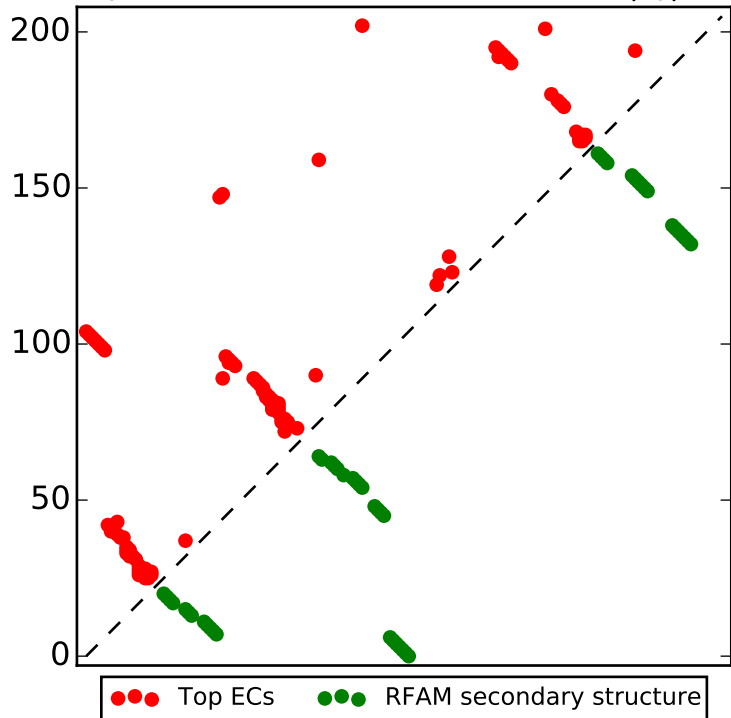
Top L/2 contacts for RF00045 with |i-j| > 4
