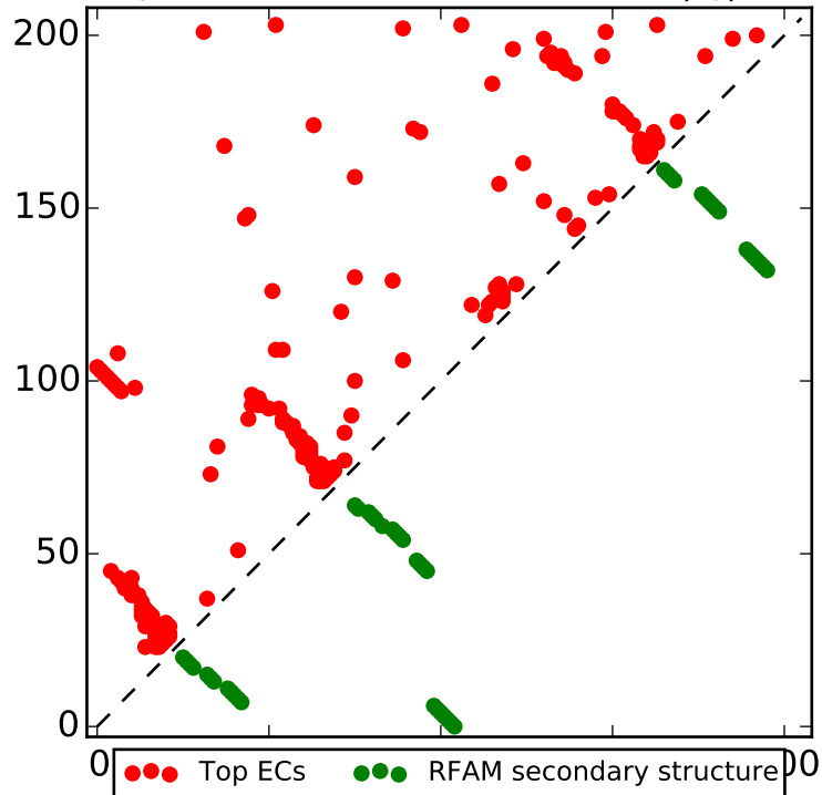
Top L contacts for RF00045 with |i-j| > 4
