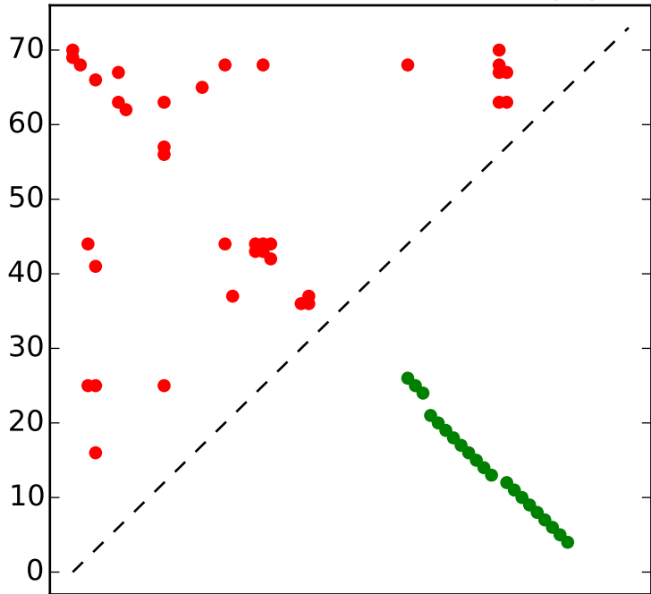
Top L/2 contacts for RF00047 with |i-j| > 4
