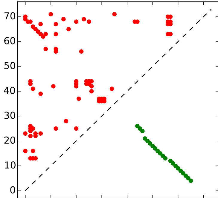
Top L contacts for RF00047 with |i-j| > 4
