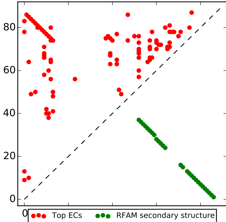
Top L contacts for RF00053 with |i-j| > 4
