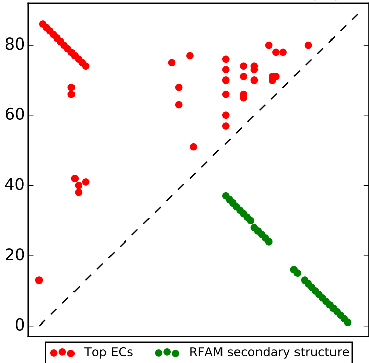
Top L/2 contacts for RF00053 with |i-j| > 4
