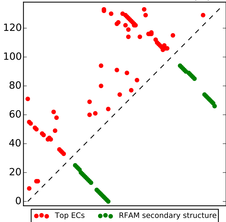
Top L/2 contacts for RF00056 with |i-j| > 4
