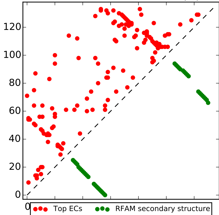
Top L contacts for RF00056 with |i-j| > 4
