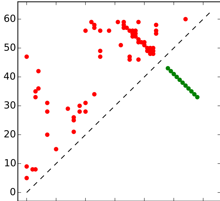
Top L contacts for RF00066 with |i-j| > 4
