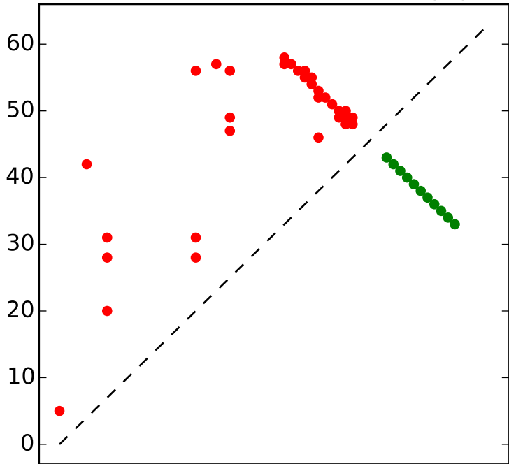
Top L/2 contacts for RF00066 with |i-j| > 4
