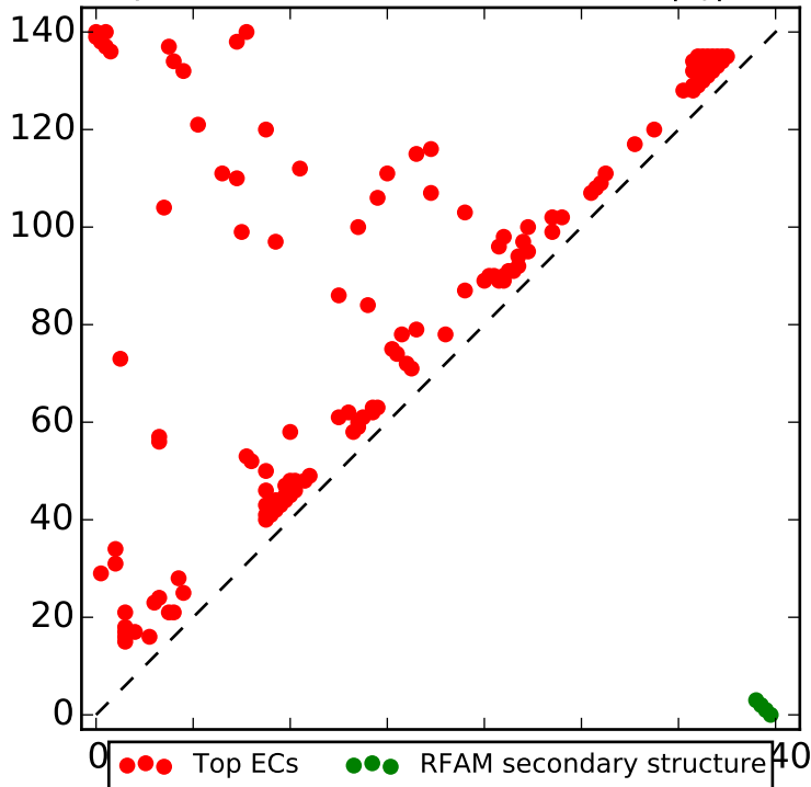
Top L contacts for RF00067 with |i-j| > 4
