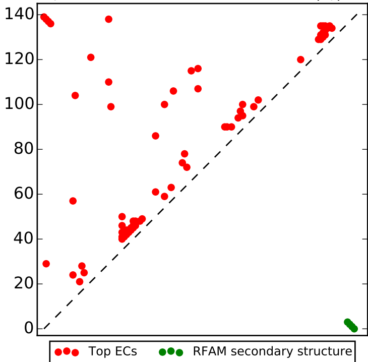
Top L/2 contacts for RF00067 with |i-j| > 4
