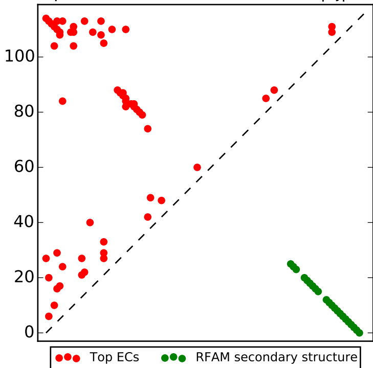
Top L/2 contacts for RF00075 with |i-j| > 4
