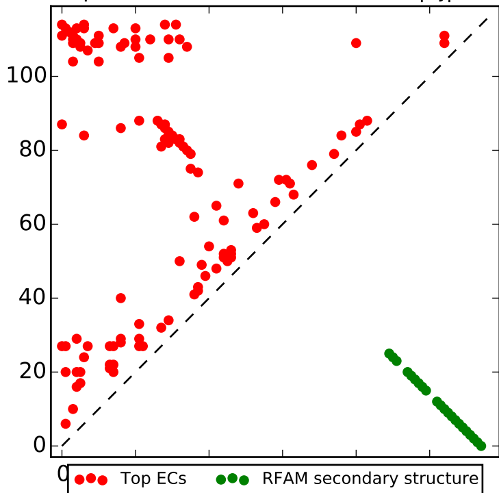
Top L contacts for RF00075 with |i-j| > 4
