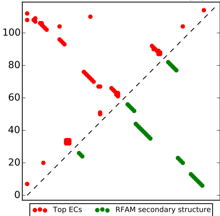
Top L/2 contacts for RF00080 with |i-j| > 4
