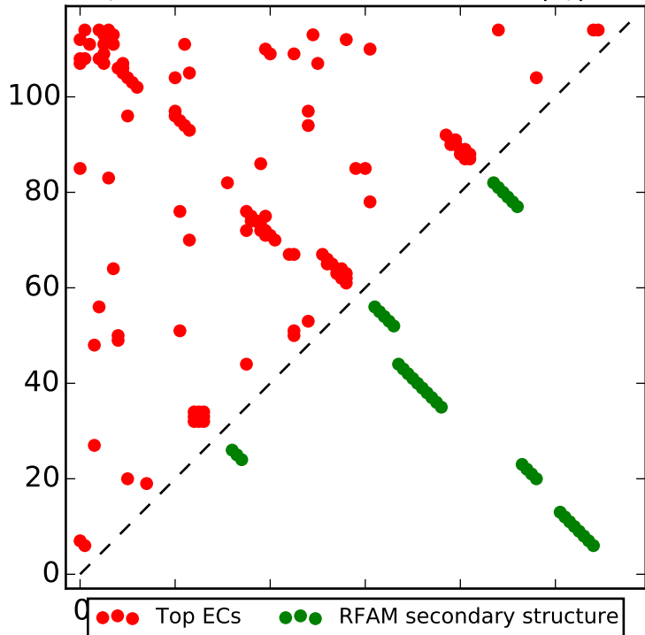
Top L contacts for RF00080 with |i-j| > 4
