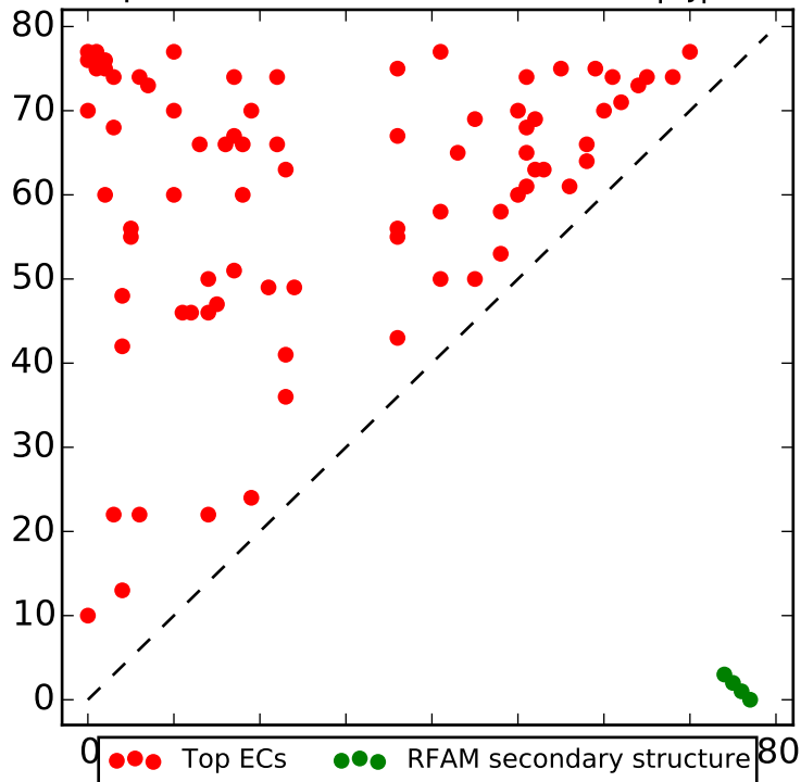
Top L contacts for RF00086 with |i-j| > 4
