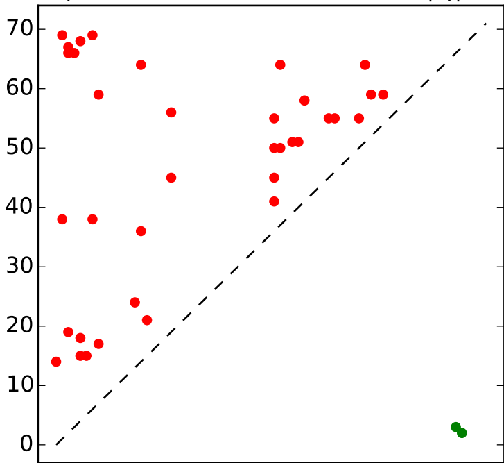
Top L/2 contacts for RF00089 with |i-j| > 4
