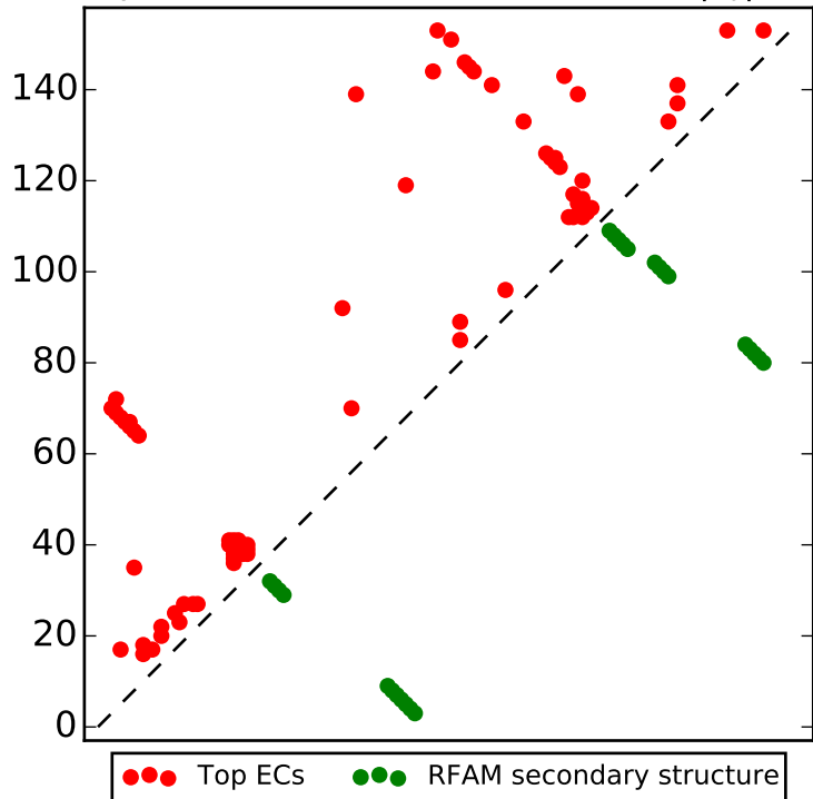
Top L/2 contacts for RF00091 with |i-j| > 4
