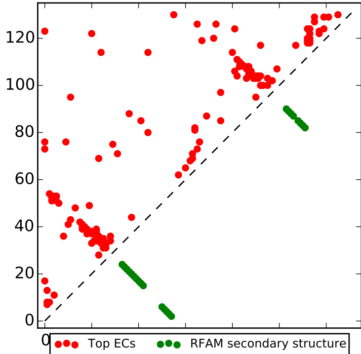
Top L contacts for RF00092 with |i-j| > 4
