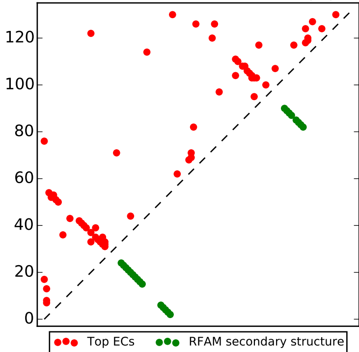
Top L/2 contacts for RF00092 with |i-j| > 4
