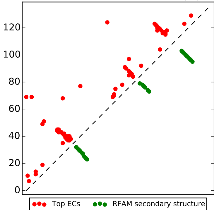
Top L/2 contacts for RF00096 with |i-j| > 4
