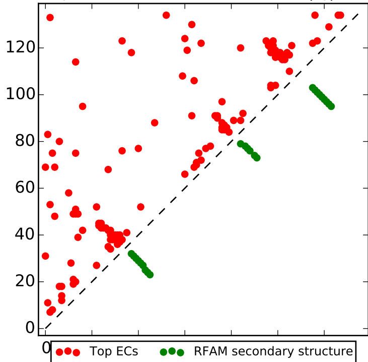
Top L contacts for RF00096 with |i-j| > 4
