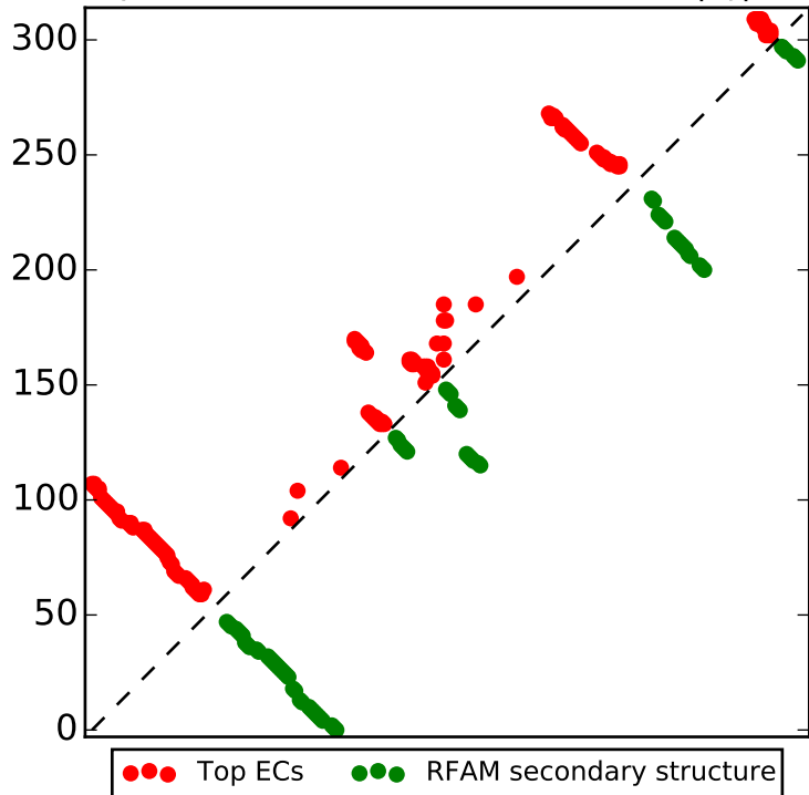
Top L/2 contacts for RF00100 with |i-j| > 4
