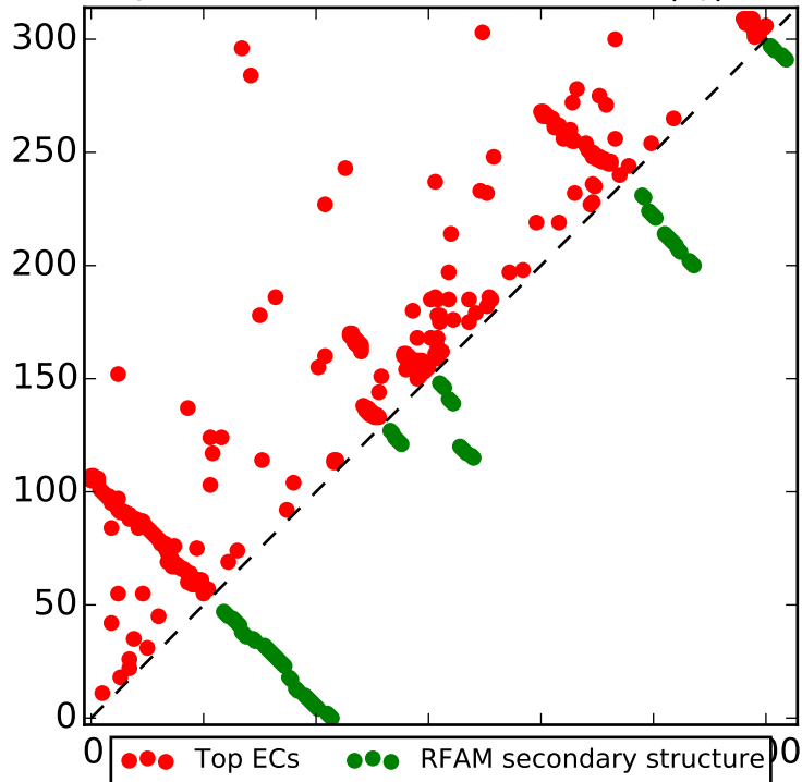
Top L contacts for RF00100 with |i-j| > 4
