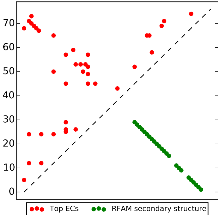
Top L/2 contacts for RF00104 with |i-j| > 4
