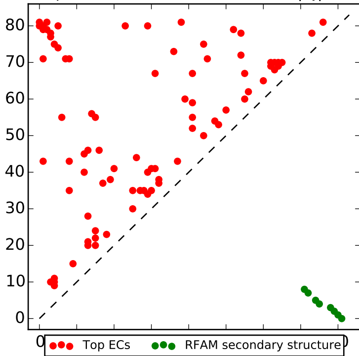
Top L contacts for RF00105 with |i-j| > 4
