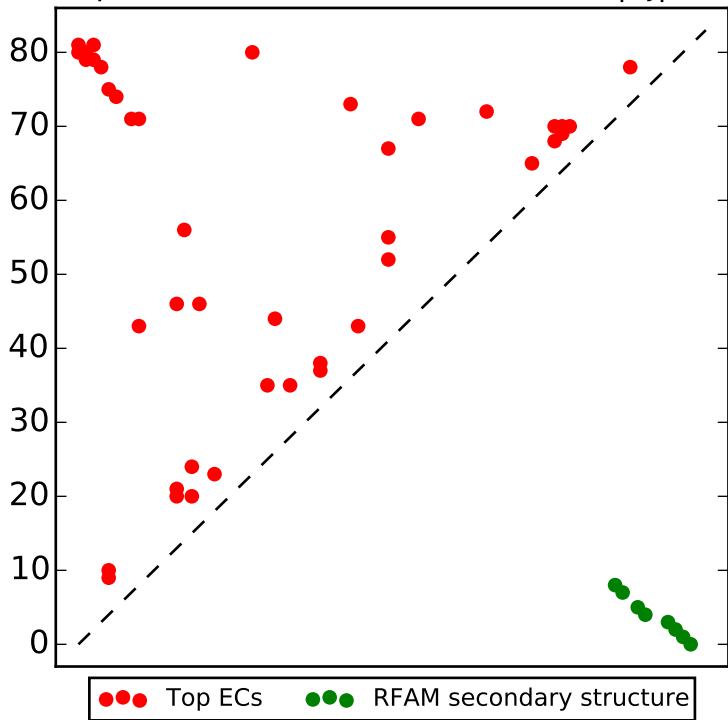
Top L/2 contacts for RF00105 with |i-j| > 4
