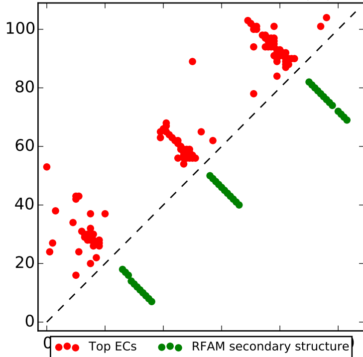
Top L contacts for RF00106 with |i-j| > 4
