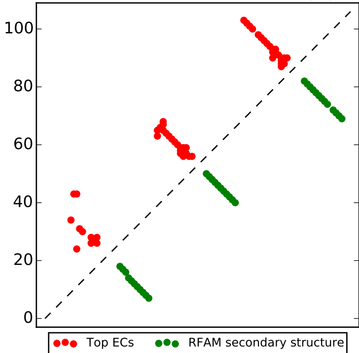
Top L/2 contacts for RF00106 with |i-j| > 4
