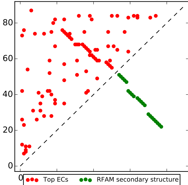
Top L contacts for RF00127 with |i-j| > 4
