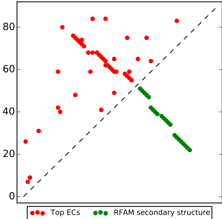
Top L/2 contacts for RF00127 with |i-j| > 4
