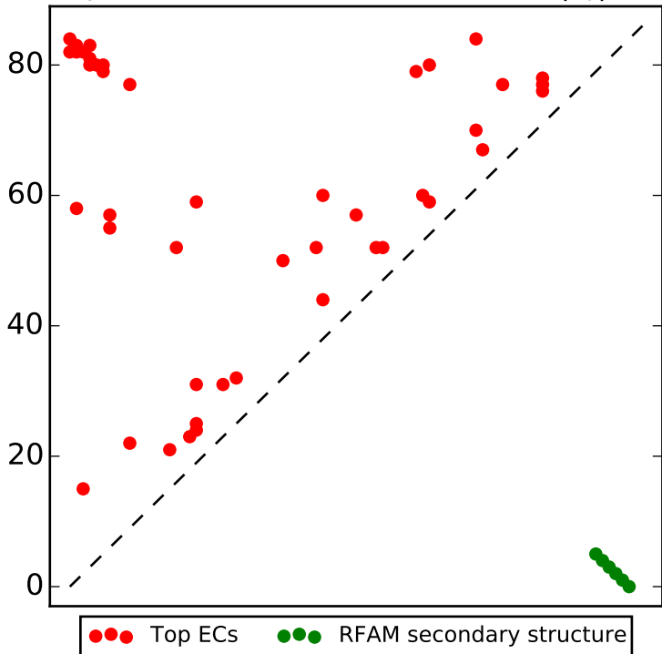
Top L/2 contacts for RF00133 with |i-j| > 4
