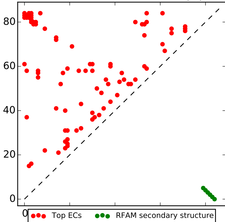
Top L contacts for RF00133 with |i-j| > 4
