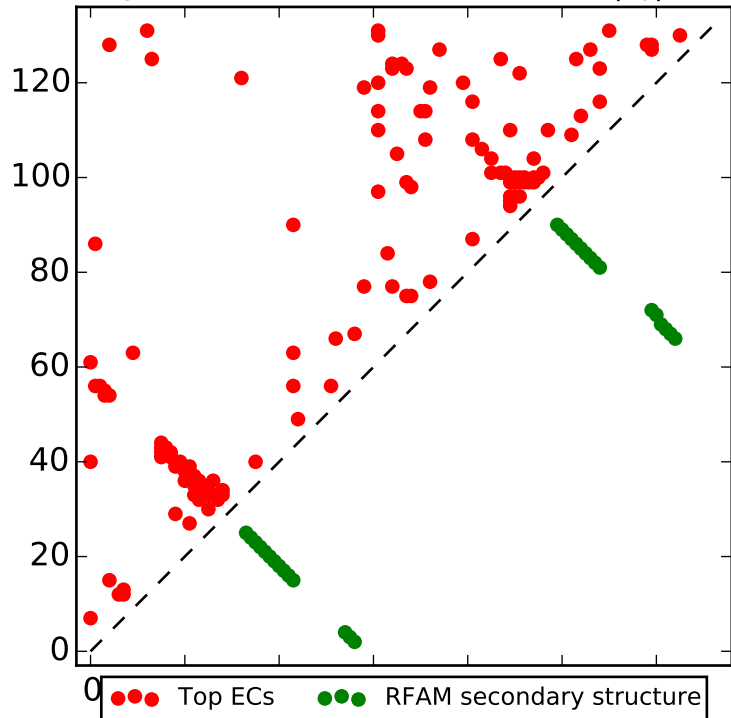
Top L contacts for RF00139 with |i-j| > 4
