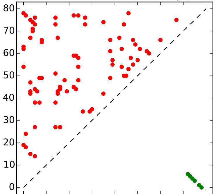
Top L contacts for RF00147 with |i-j| > 4
