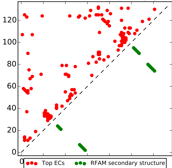
Top L contacts for RF00155 with |i-j| > 4
