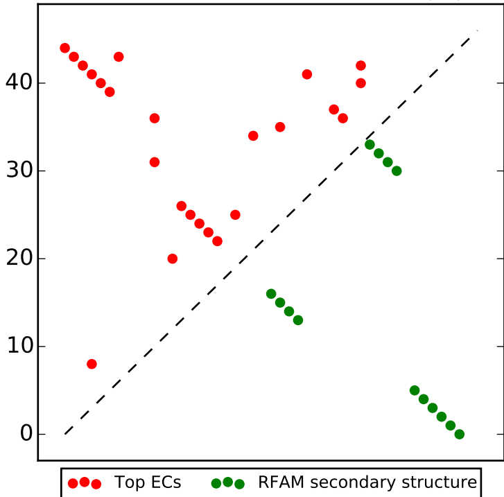
Top L/2 contacts for RF00163 with |i-j| > 4
