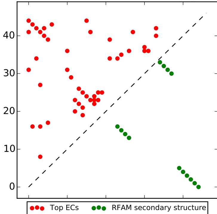
Top L contacts for RF00163 with |i-j| > 4
