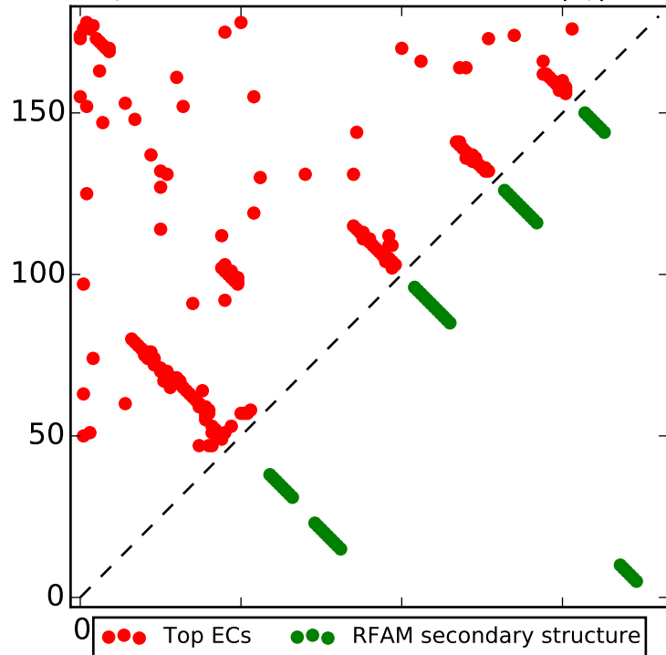
Top L contacts for RF00168 with |i-j| > 4
