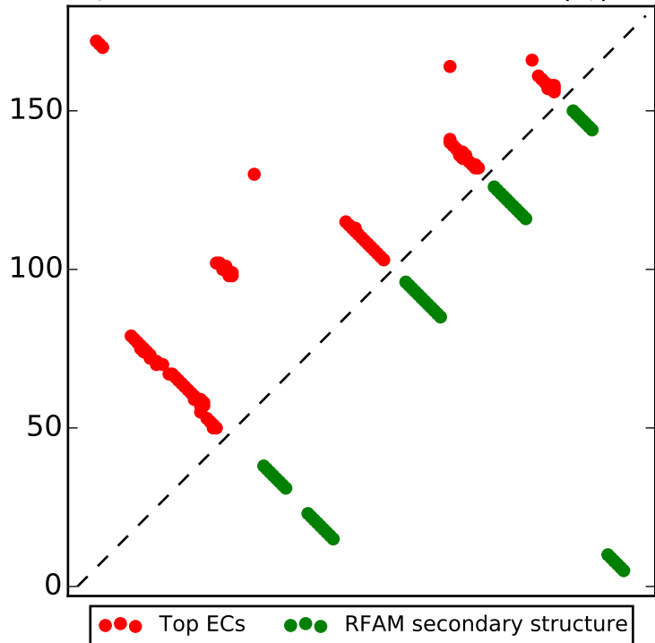
Top L/2 contacts for RF00168 with |i-j| > 4
