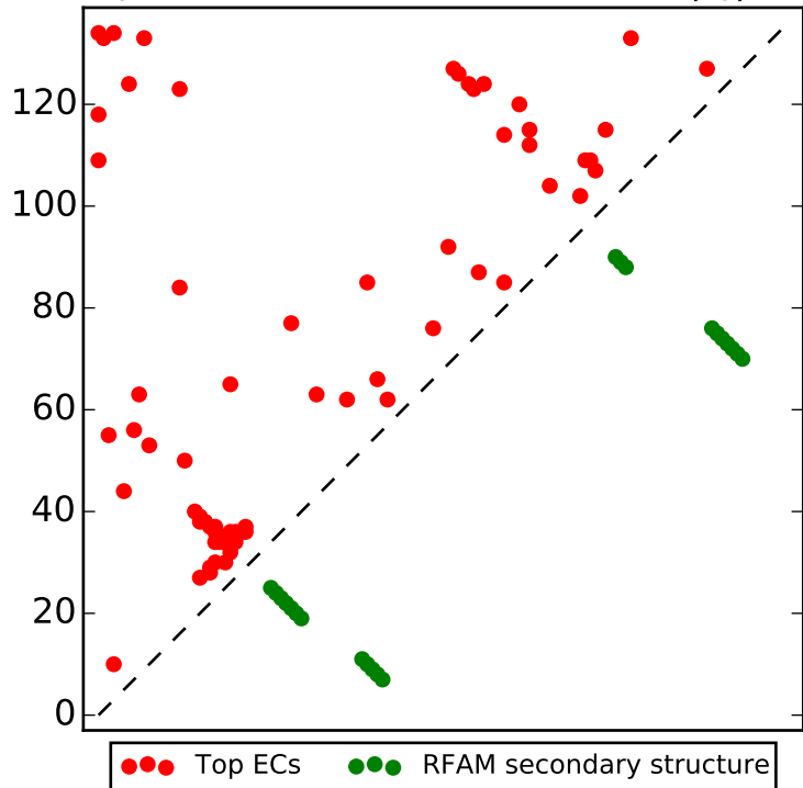
Top L/2 contacts for RF00190 with |i-j| > 4
