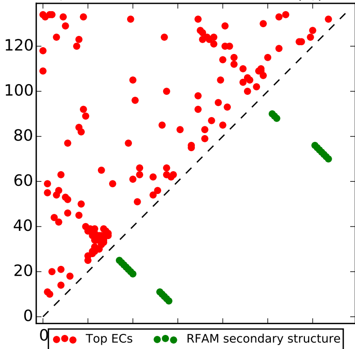
Top L contacts for RF00190 with |i-j| > 4
