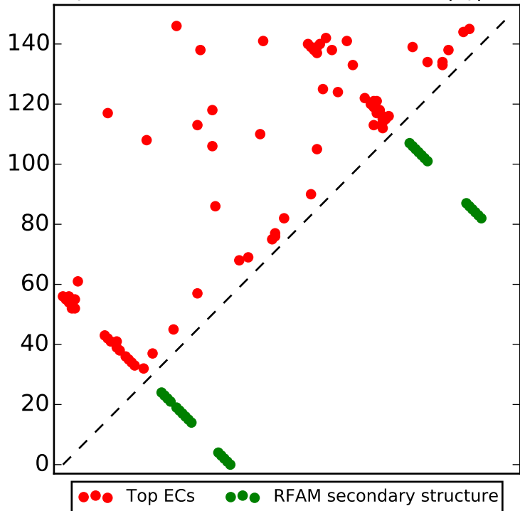
Top L/2 contacts for RF00191 with |i-j| > 4
