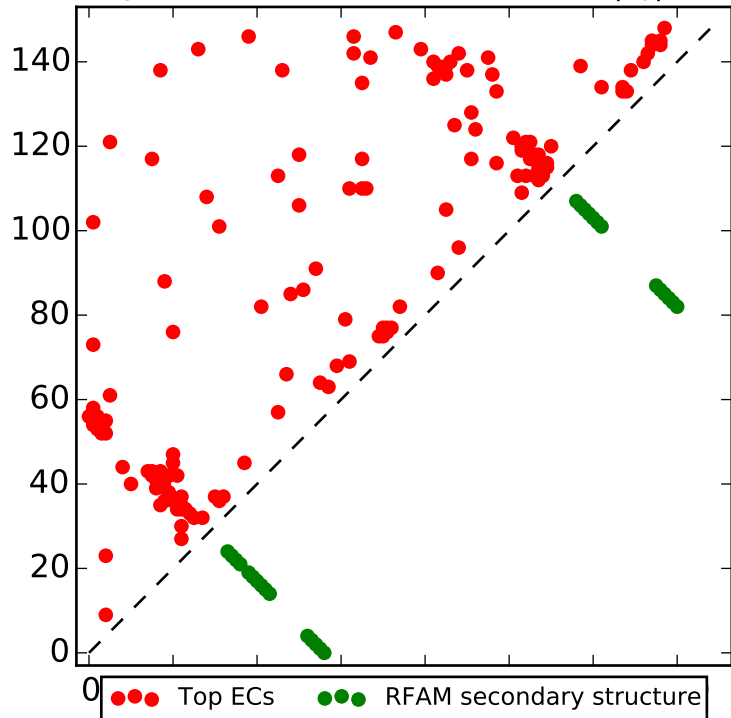
Top L contacts for RF00191 with |i-j| > 4
