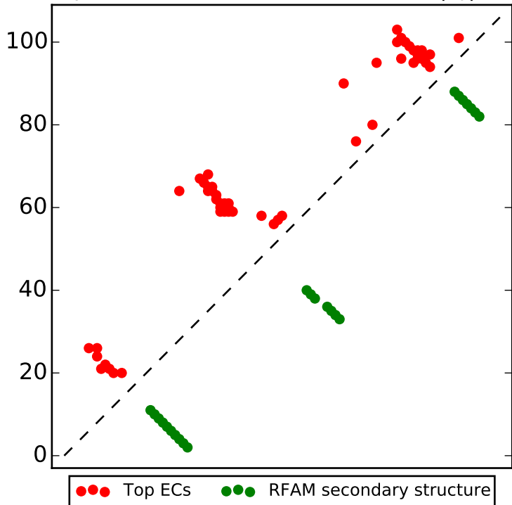
Top L/2 contacts for RF00198 with |i-j| > 4
