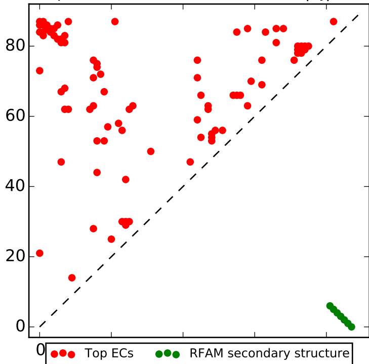
Top L contacts for RF00213 with |i-j| > 4
