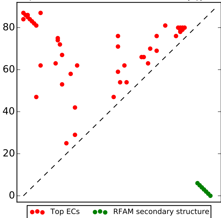
Top L/2 contacts for RF00213 with |i-j| > 4
