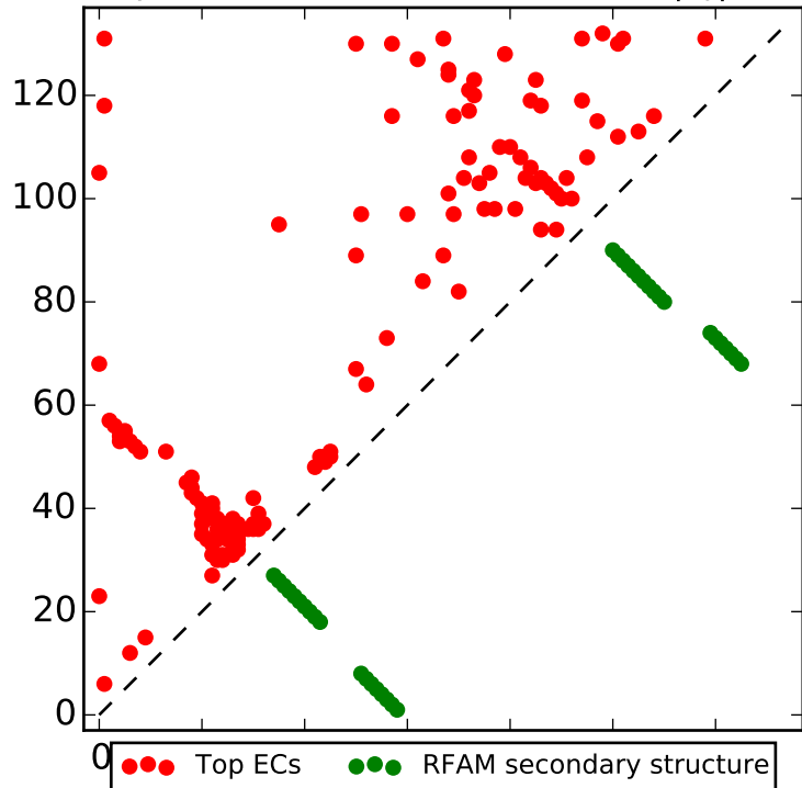
Top L contacts for RF00263 with |i-j| > 4
