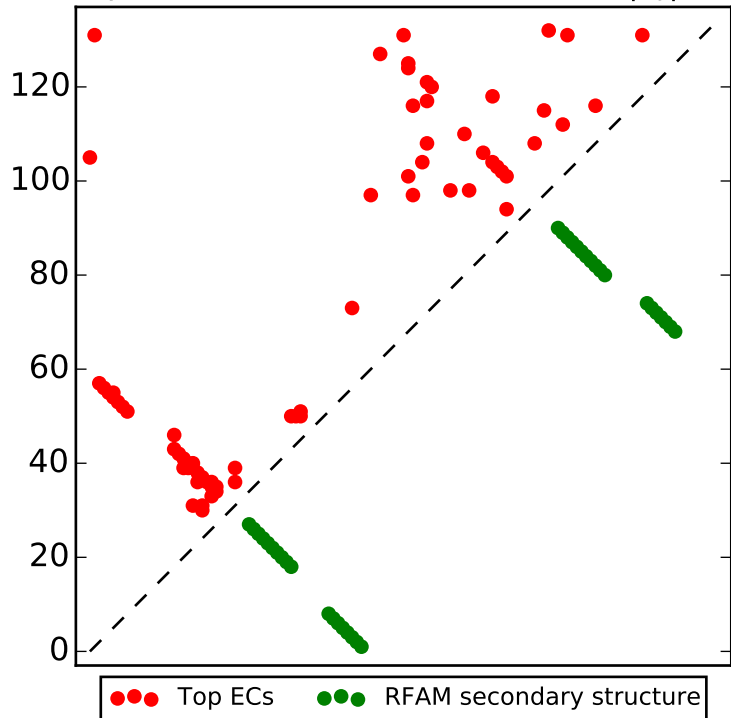
Top L/2 contacts for RF00263 with |i-j| > 4
