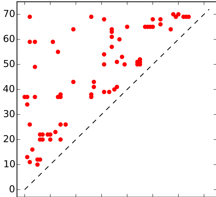
Top L contacts for RF00277 with |i-j| > 4
