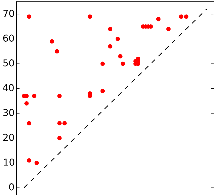
Top L/2 contacts for RF00277 with |i-j| > 4
