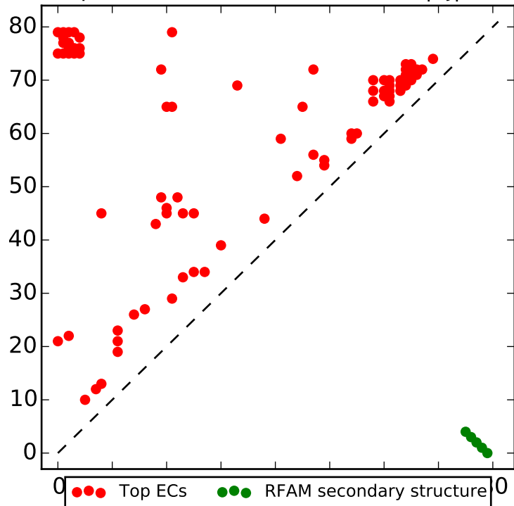
Top L contacts for RF00284 with |i-j| > 4
