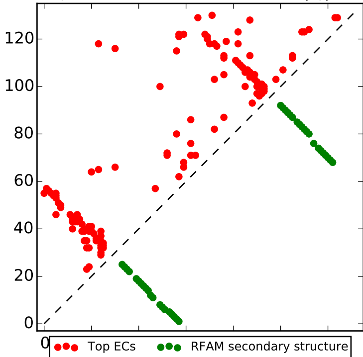
Top L contacts for RF00334 with |i-j| > 4
