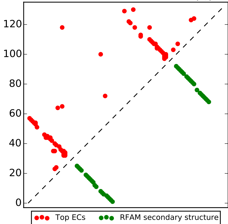
Top L/2 contacts for RF00334 with |i-j| > 4
