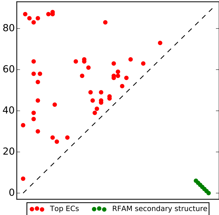
Top L/2 contacts for RF00343 with |i-j| > 4
