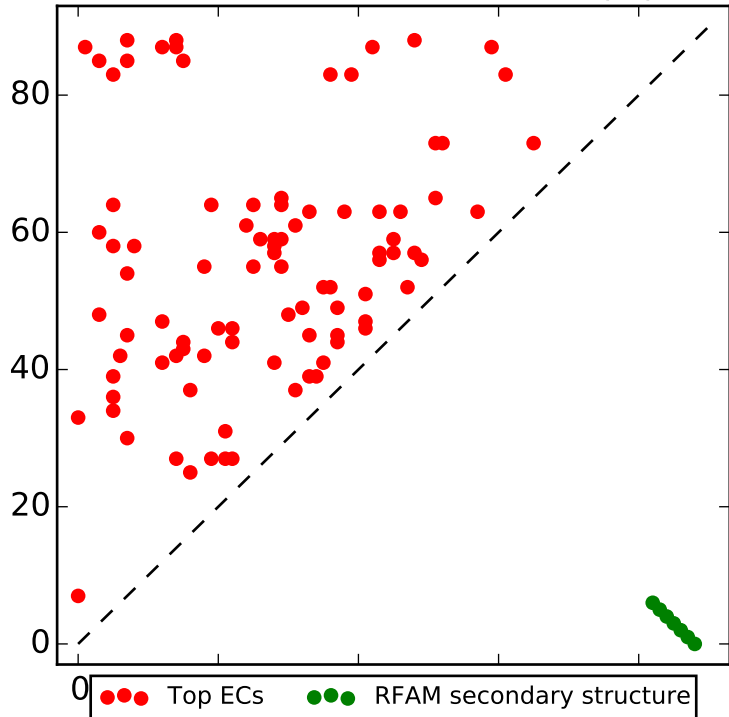
Top L contacts for RF00343 with |i-j| > 4
