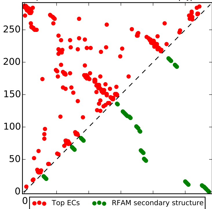
Top L contacts for RF00373 with |i-j| > 4
