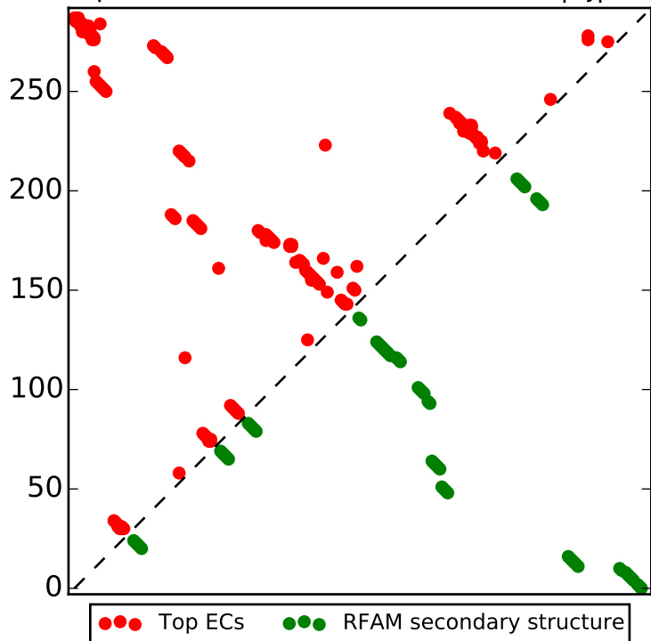
Top L/2 contacts for RF00373 with |i-j| > 4
