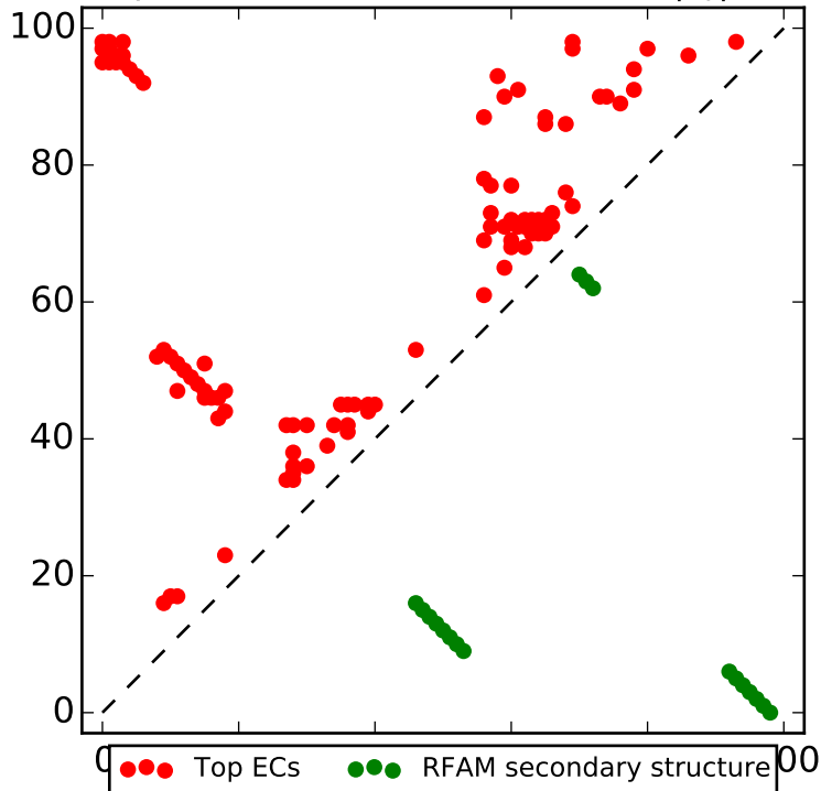
Top L contacts for RF00375 with |i-j| > 4
