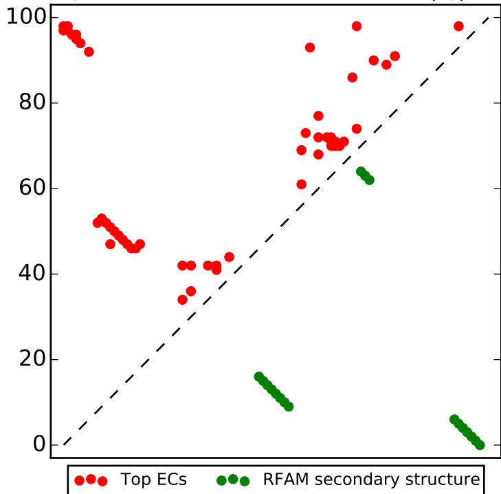
Top L/2 contacts for RF00375 with |i-j| > 4
