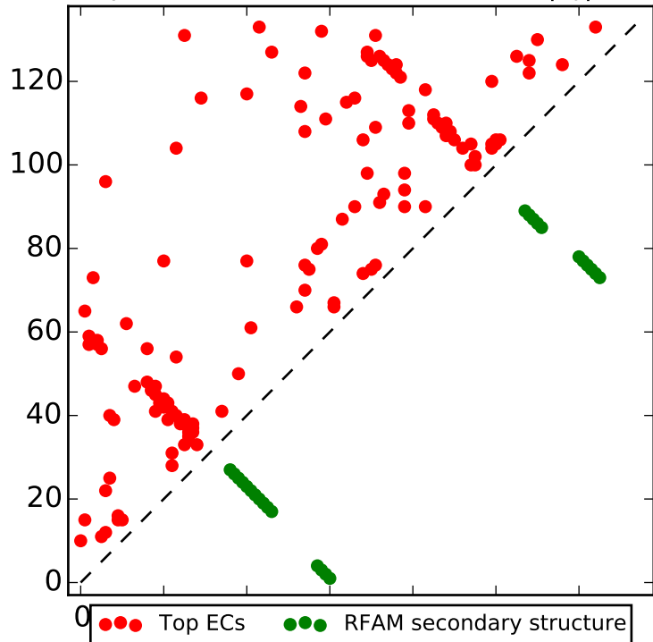
Top L contacts for RF00392 with |i-j| > 4
