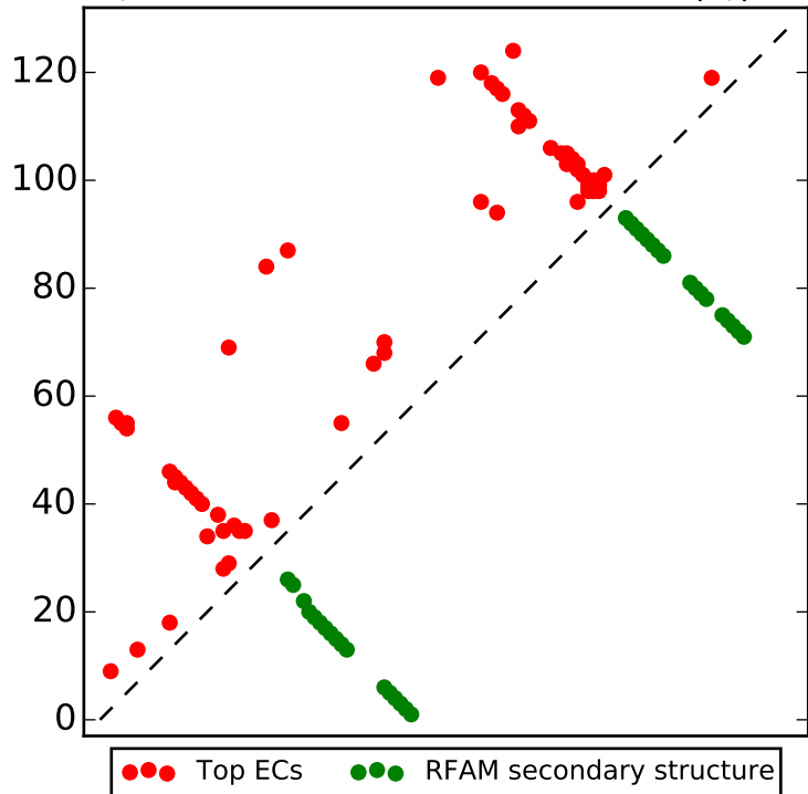
Top L/2 contacts for RF00402 with |i-j| > 4
