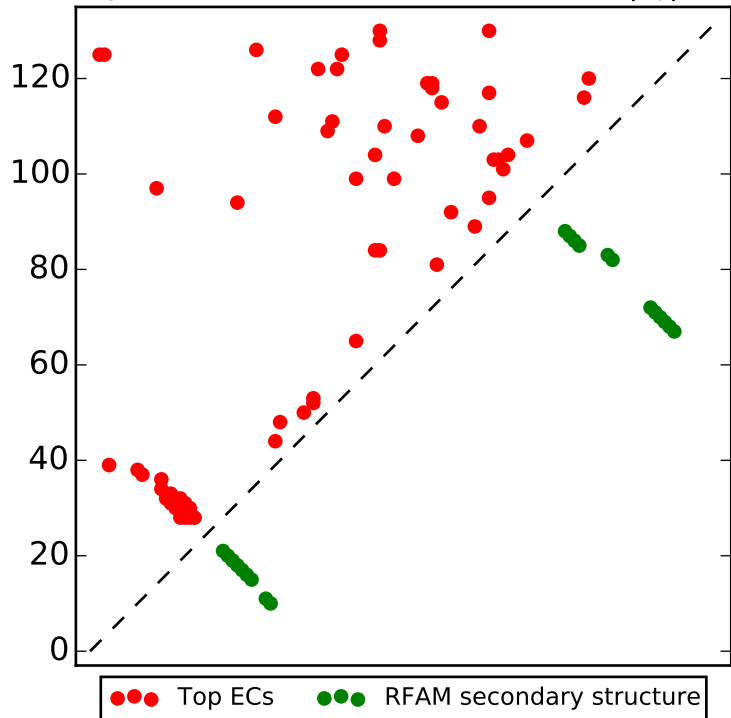
Top L/2 contacts for RF00405 with |i-j| > 4
