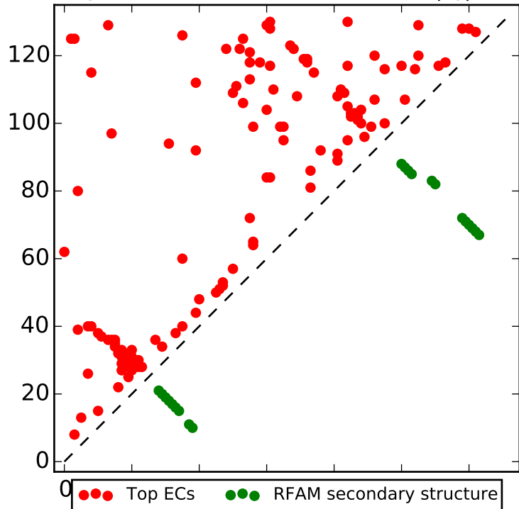
Top L contacts for RF00405 with |i-j| > 4
