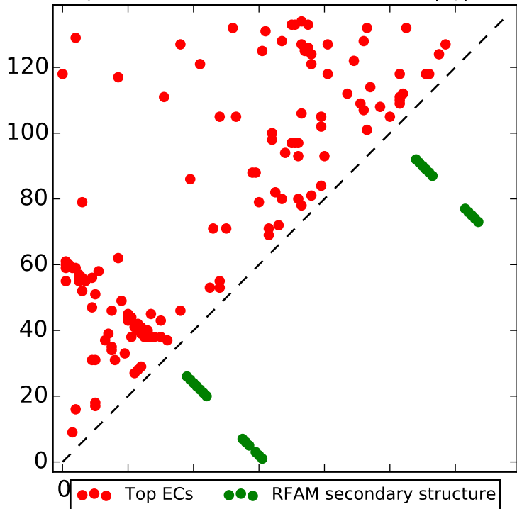
Top L contacts for RF00408 with |i-j| > 4
