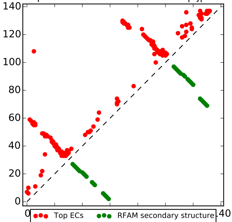
Top L contacts for RF00409 with |i-j| > 4
