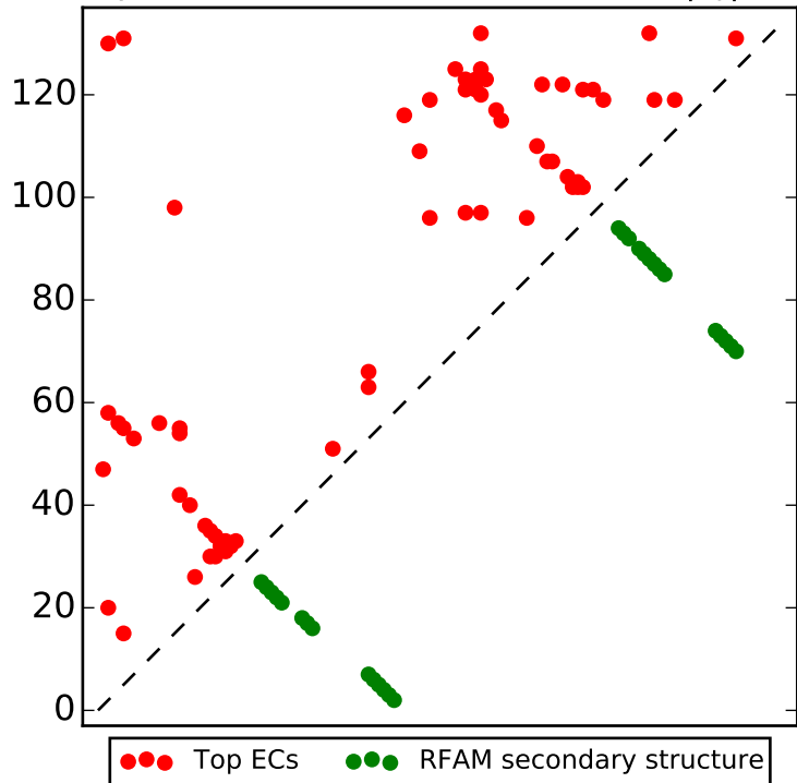
Top L/2 contacts for RF00411 with |i-j| > 4
