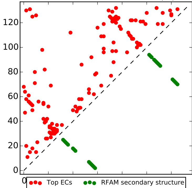
Top L contacts for RF00411 with |i-j| > 4
